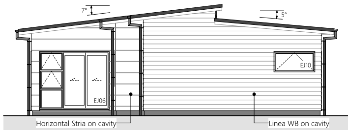
3 West Elevation
