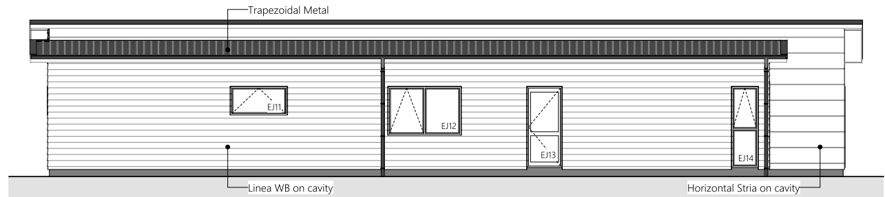
4 South Elevation
