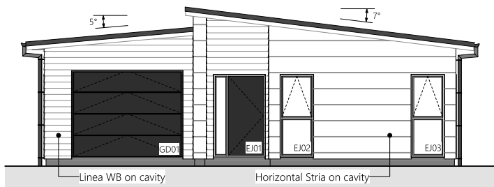
1 East Elevation
