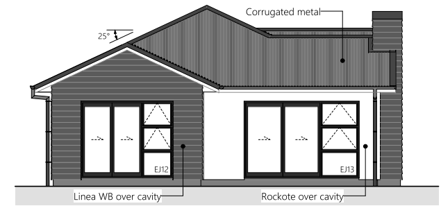
4 East Elevation
