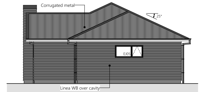
2 West Elevation
