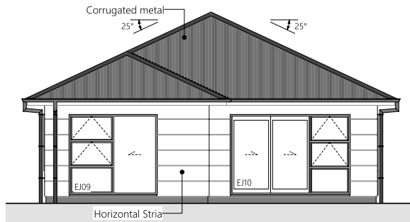
3 Elevation Three
