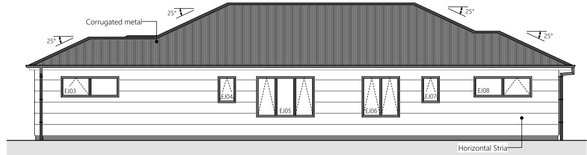
2 Elevation Two
