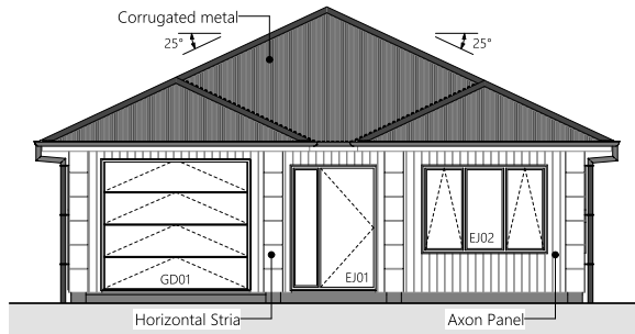
1 Elevation One
