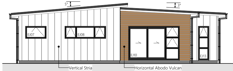
3 North Elevation
