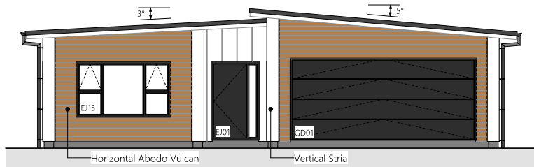
1 South Elevation
