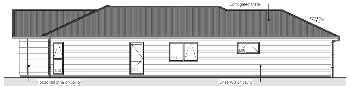
2 South Elevation
