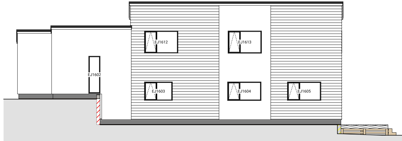
2 Lot 16 - North Elevation
