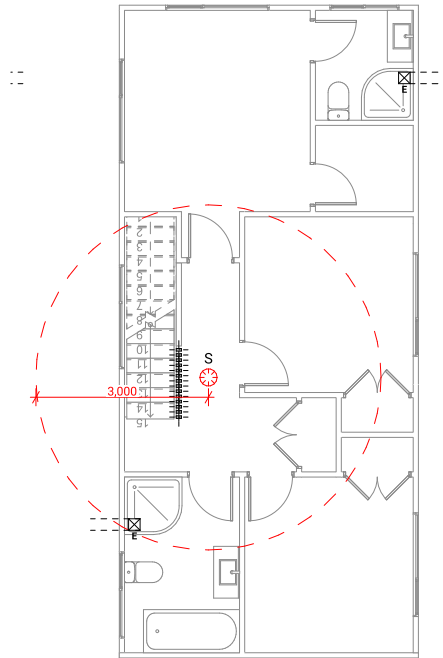
Upper Electrical Plan
