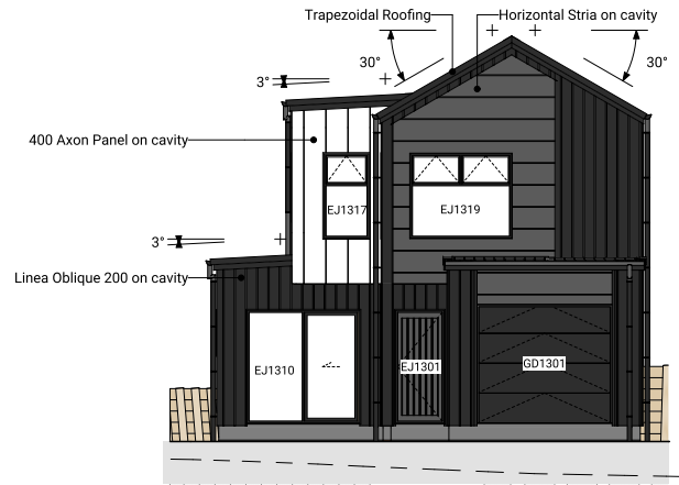
1 Lot 13 - West Elevation
