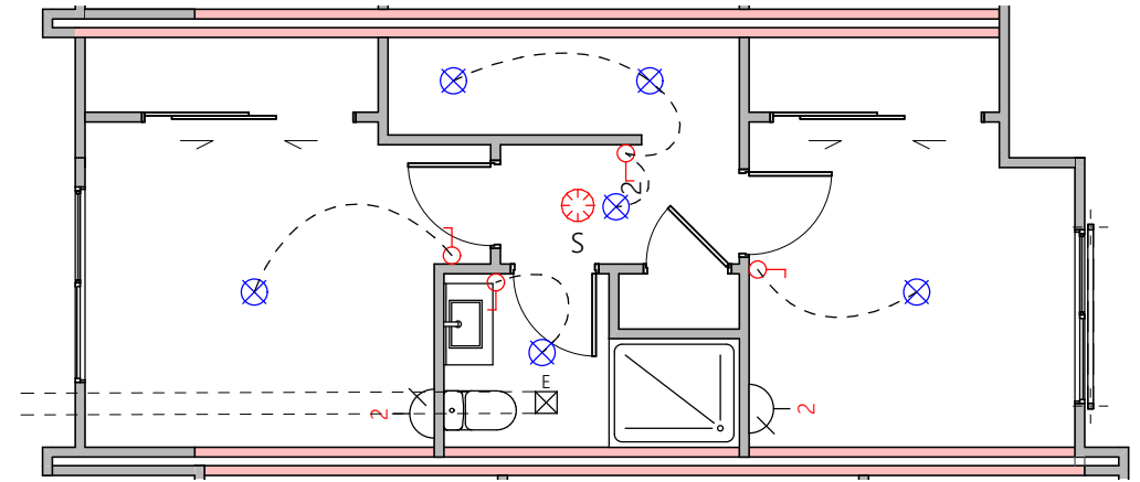
Upper Electrical Plan
