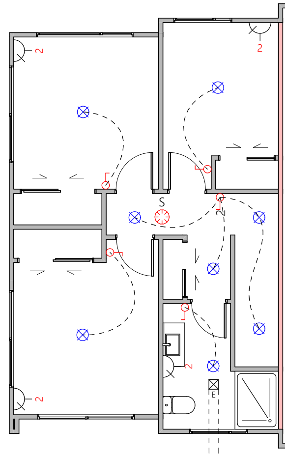
Upper Electrical Plan
