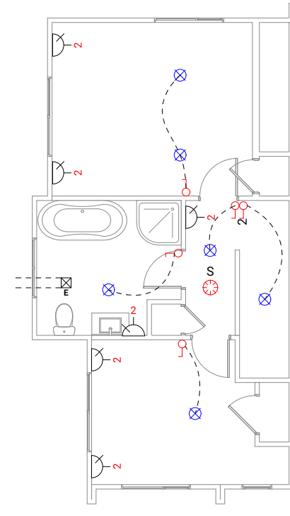
Upper Electrical Plan
