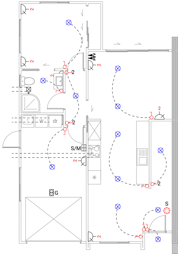
Lower Electrical Plan
