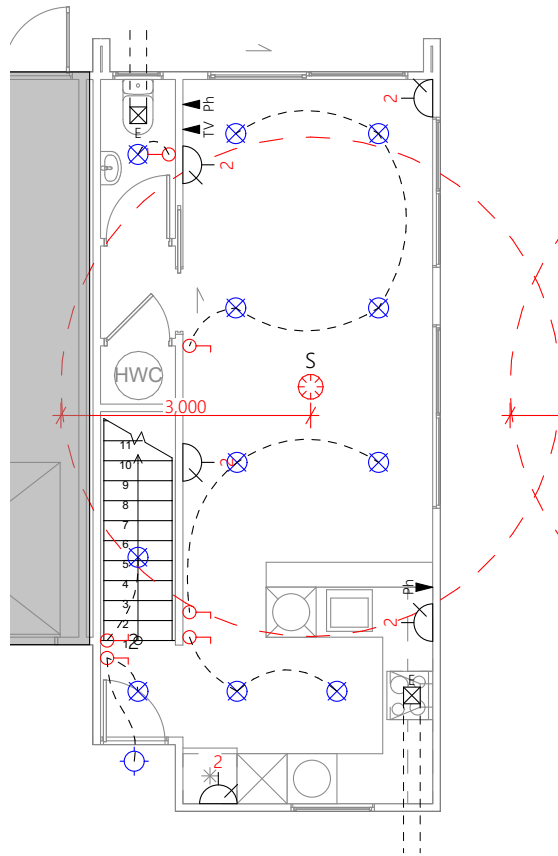
Lower Electrical Plan
